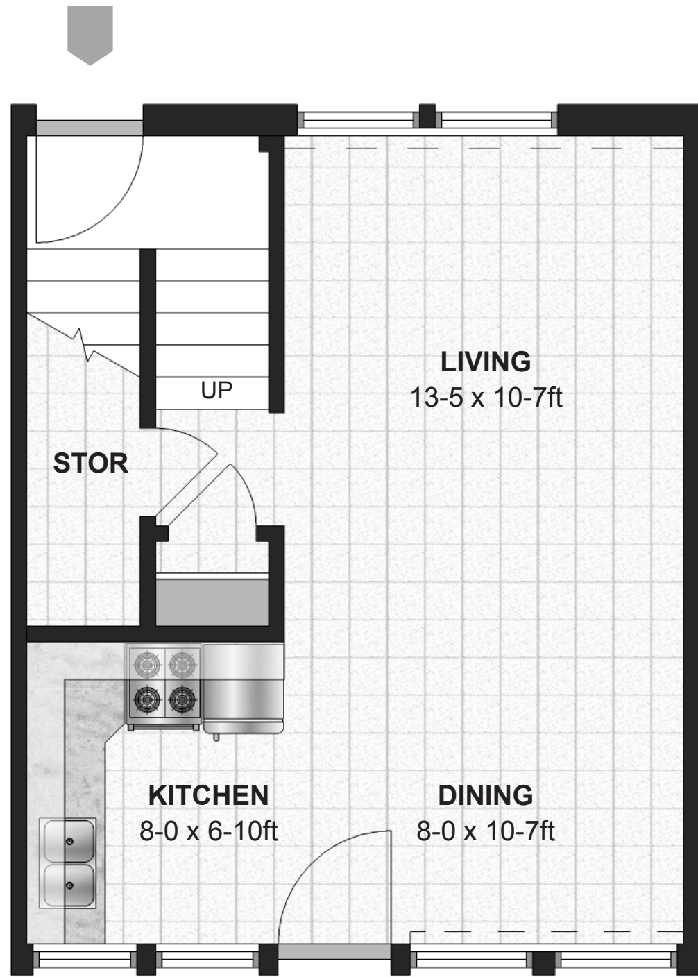
1 st FLOOR
